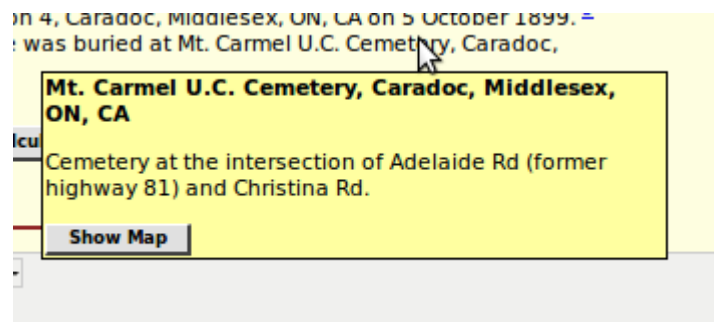
Illustration 4: Location Popup
